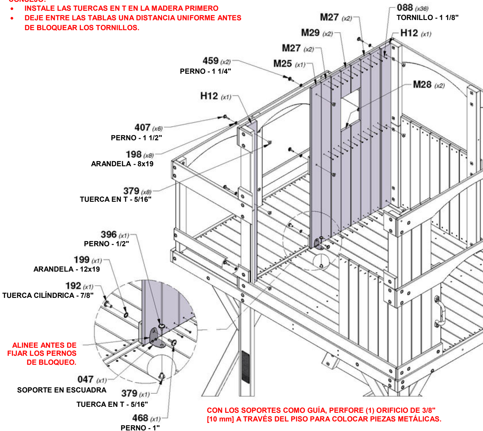
M28 TABLA DE PARED - W4L06535 (x2) 5/8"x3 3/8"x29 7/8" (16x86x760)
